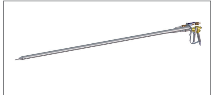
Hand lance with gun 1800 mm long Order No. 0656948
