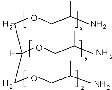
Figure 7: Polyoxypropylene Triamine Structure Polyether Triamine
